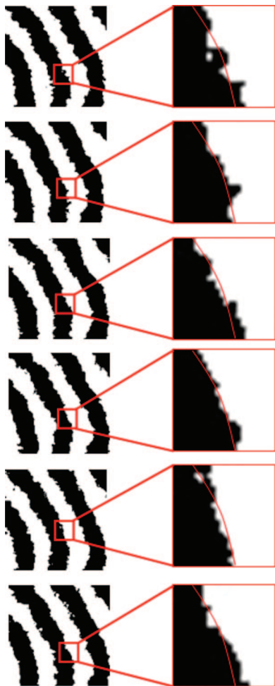
Figure 6. AFM images of a 100 \times 100 \text{ nm}^2 , with a 10 \times 10 \text{ nm}^2 region magnified, showing the PMMA/PS boundary. The images were taken 30 s apart and show that protrusions of the PMMA (black) domain are followed by retractions, indicating that there is a restoring force. Since the force is isotropic, it cannot be due to some larger scale flows. Curvature minimization is thus the likeliest force responsible.
