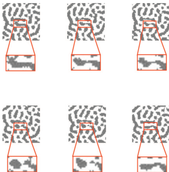
Figure 5. AFM images of a 200 \times 200 \text{ nm}^2 PMMA/PS boundary. The images were taken 30 s apart and show that protrusions of the PMMA (black) domain are followed by retractions, indicating that there is a restoring force. Since the force is isotropic, it cannot be due to some larger scale flows. Curvature minimization is thus the likeliest force responsible.
