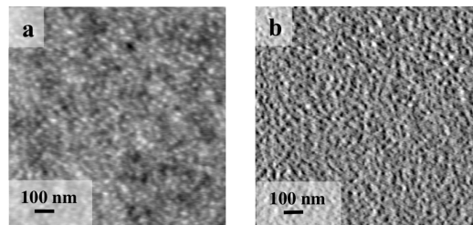
Figure 1. AFM height (a) and phase (b) images of PS- b -PMMA at 373 K without a prior anneal. PMMA domains appear in white in the height image, as they are raised compared to the matrix, and in black in the phase.
