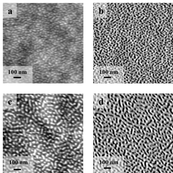
Figure 2. AFM height (a, c) and their corresponding phase (b, d) images of PS- b -PMMA at 398 K, without a prior high-temperature anneal. The images were taken 8 min apart, the first image being taken within 5 min of reaching that temperature. The ramp rate was 20 K/min. The average interdomain spacing is 35 nm in (a, b) and 40 nm in (c, d).
