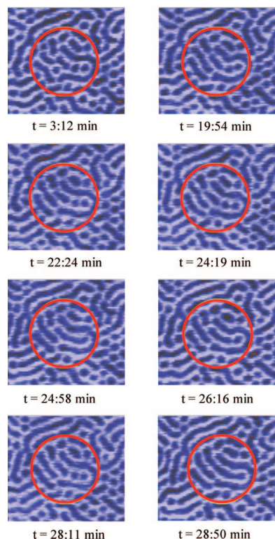
Figure 4. AFM images of PMMA domains joining and breaking up at a fixed temperature (448 K). In the circled region, four separate domains join into one via a series of joints and breaks. The images are 500 \times 450 \text{ nm}^2 .
